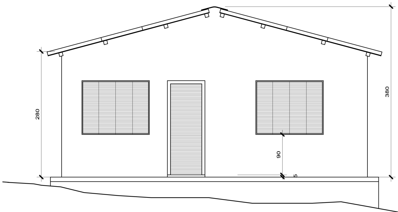
FACHADA PRINCIPAL
