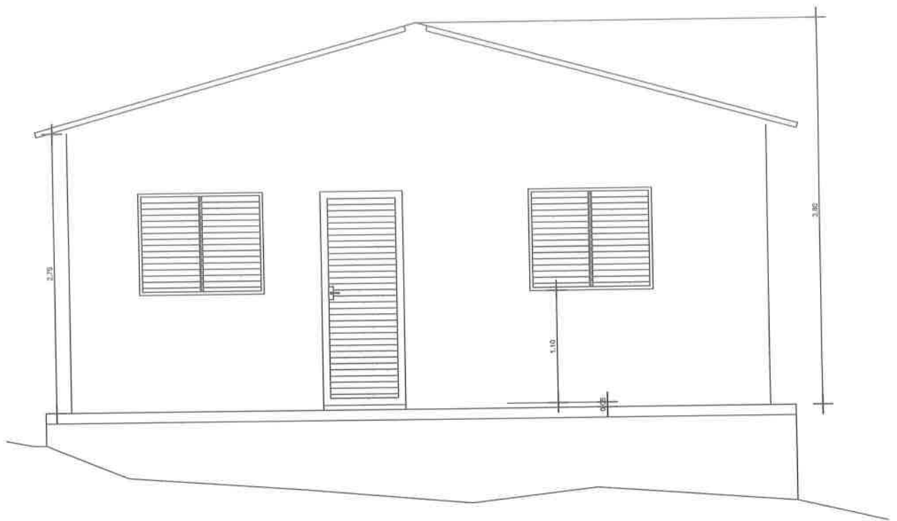
FACHADA PRINCIPAL
